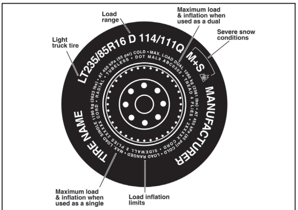
Figure 4: Typical Light Truck Tire Markings
