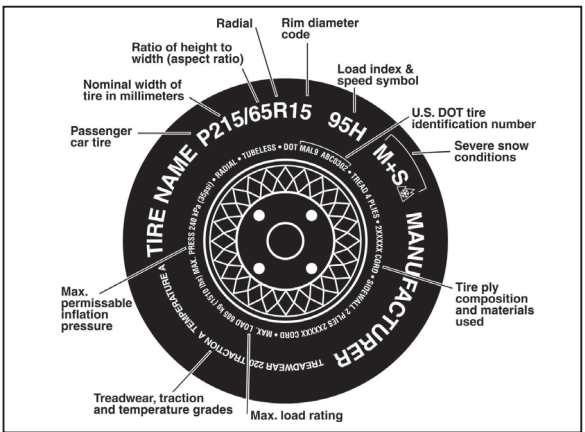
Figure 3: Typical Passenger Tire Markings
